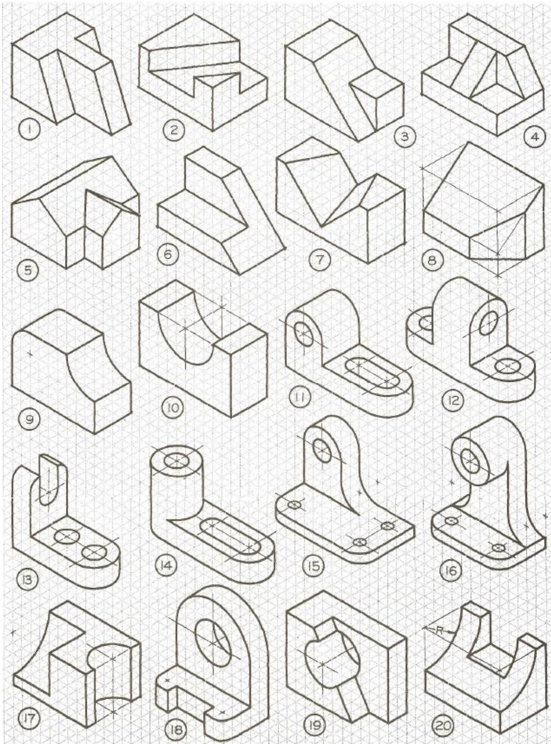
Fig. 7-28. Sketching problems. See instructions referring to Fig. 7-26.
